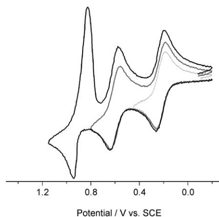
Figure 3. CVs at different potential scan reversals of 1.0 \times 10^{-3} M 1 in CH 2 Cl 2 at a Au disk electrode ( d = 0.5 mm); scan rate: 0.5 V s –1 ; T : 20^\circ\text{C} .
